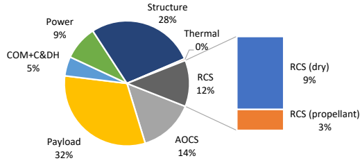
Figure 3: ALE-2 Bus-system Configuration
