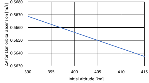
Figure 11: Delta V Required for 1-km Orbital Ascension
